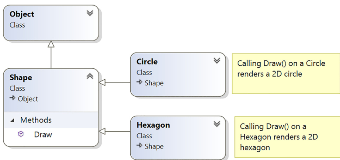
Figure 5-3. Classical polymorphism
