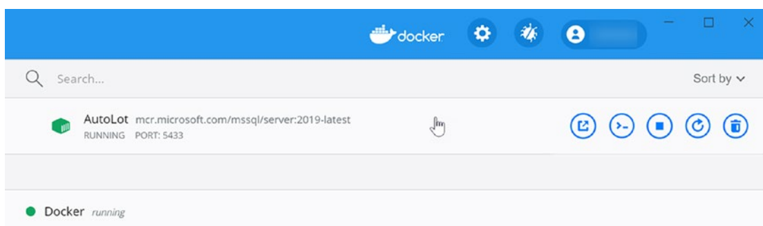
Figure 20-2. Docker Dashboard
